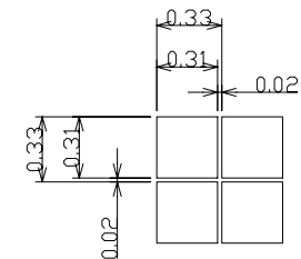
DETAIL OF DOTS: SCALE 10:1
